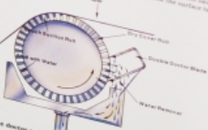
Double doctor removes water, fines and fibres from couch roll.
